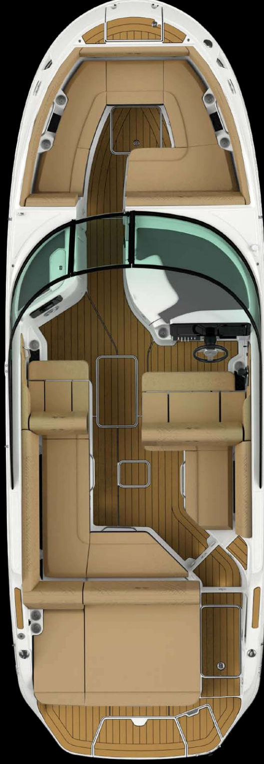
DECK / COCKPIT
